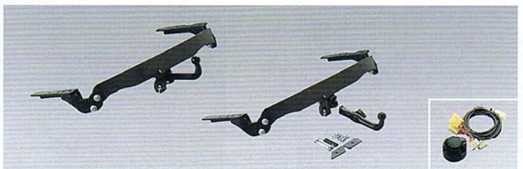
40. Trailer hitch (Fixed, Detachable), Wiring kit Towing capacity maximum 2,000 kg.
